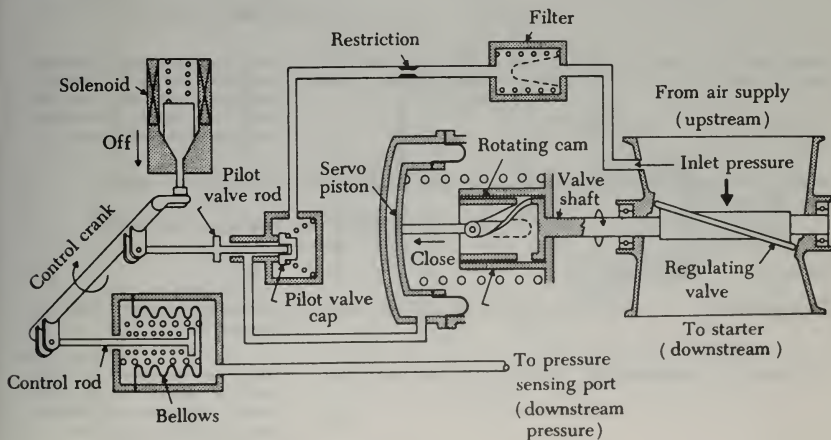
FIGURE 5-19. Pressure-regulating and shutoff valve in "off" position.
